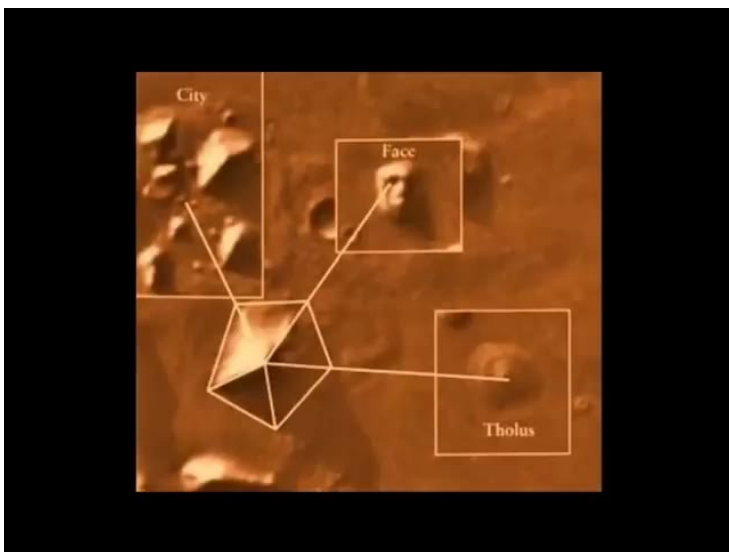
Plate 034. Mars Cydonia annotated terrain
